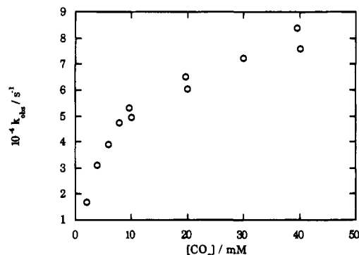
Figure 2. Kinetic behavior of the TP radical anion in the presence of \text{CO}_2 , as shown by a plot of the observed first-order rate constant vs \text{CO}_2 concentration.
