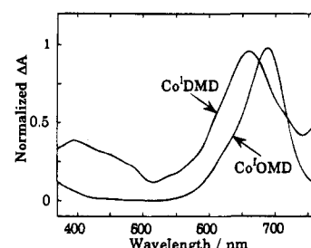
Figure 6. Transient absorption spectra of Co I DMD + and Co I OMD + . The spectrum of Co I OMD + was observed 6 μs after the excitation for the degassed sample containing 0.1 mM TP, 0.5 M TEA, 0.1 M TEAP, and 1 mM Co II OMD 2+ in MeCN/MeOH. The spectrum of Co I OMD + was observed 6 μs after the excitation for the pre-irradiated (at 313 nm, for 30 min to change from Co III DMD 3+ to Co II DMD 2+ ) sample containing 0.1 mM TP, 0.5 M TEA, 0.1 M TEAP, and 1 mM Co III DMD 3+ in MeCN/MeOH.
