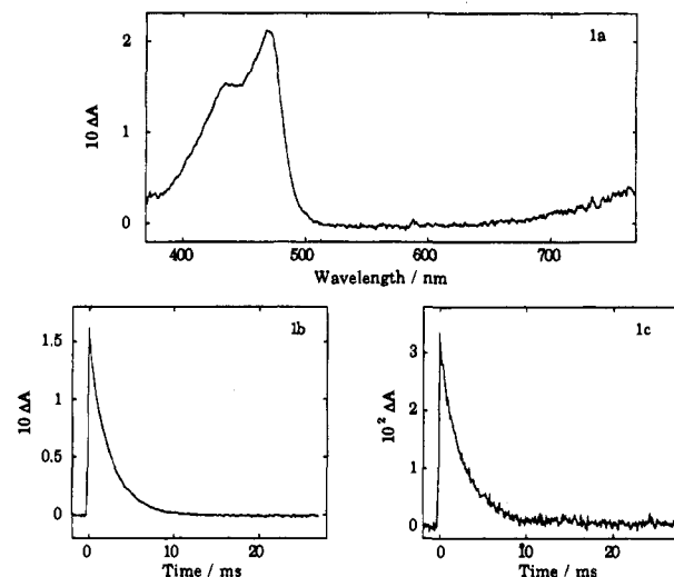
Figure 1. (a) Transient absorption spectrum of the TP radical anion observed 6 \mu\text{s} after the excitation for the degassed sample containing 0.1 mM TP, 0.5 M TEA, and 0.1 M TEAP in MeCN/MeOH. (b) Decay of \text{TP}^{\bullet-} monitored at 470 nm. (c) Decay of \text{TP}^{\bullet-} monitored at 750 nm. The first-order fitting of both curves gives the lifetime of 2.5 ms.
