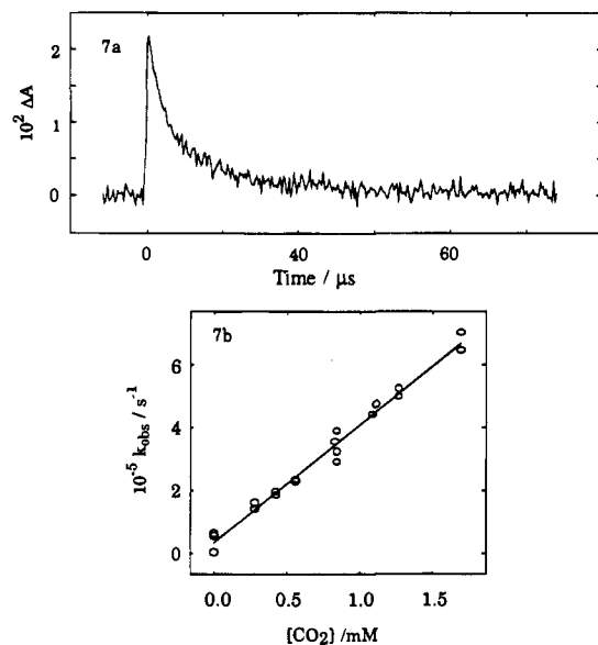
Figure 7. (a) Transient decay curve of Co I DMD + monitored at 650 nm for the sample containing 0.1 mM TP, 0.5 M TEA, 0.1 M TEAP, 1 mM Co II DMD 2+ , and 0.42 mM CO 2 in MeCN/MeOH. (b) Kinetic behavior of the Co I DMD + in the presence of CO 2 , as shown by a plot of the pseudo-first-order rate constant vs CO 2 concentration. k_{obs} = (3.7 \times 10^8)[CO_2] - (3 \pm 3) \times 10^4 (s^{-1}) .
